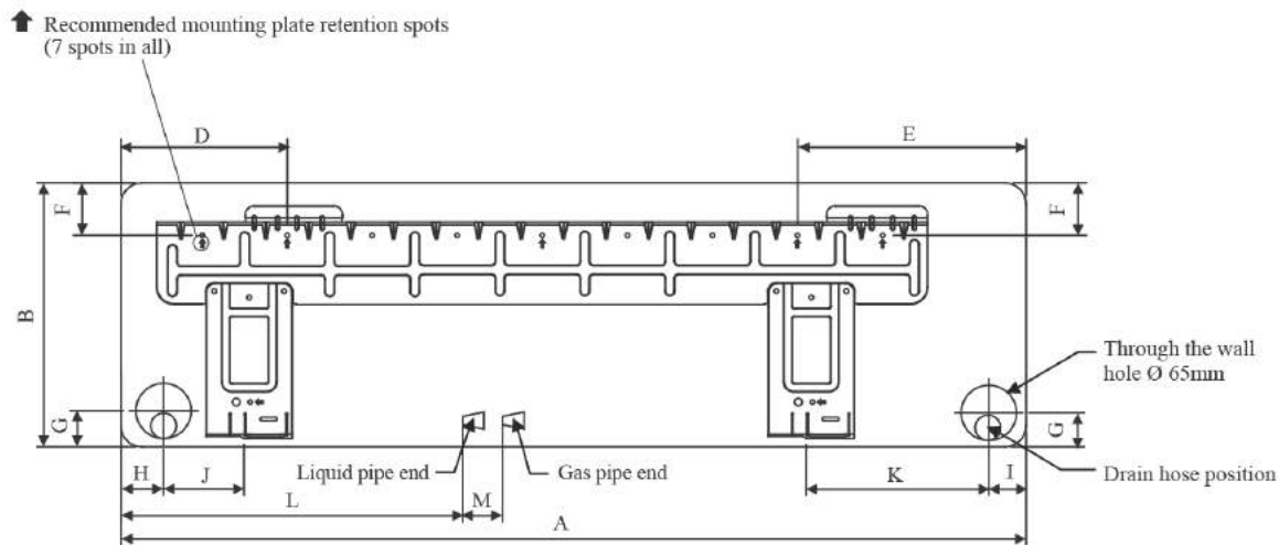
INSTALLATION PLATE 50/60
