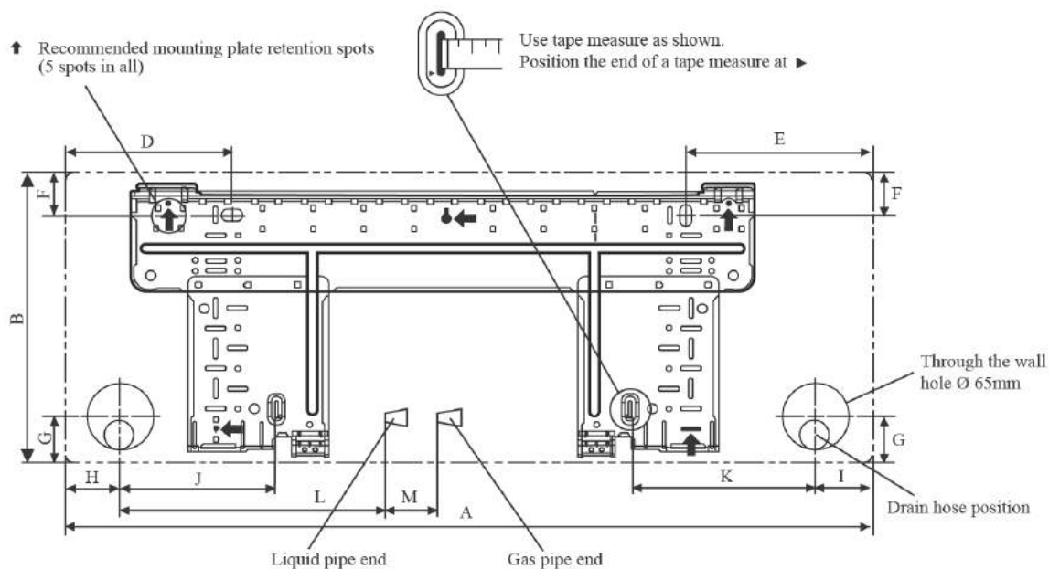
INSTALLATION PLATE 20/25/35
