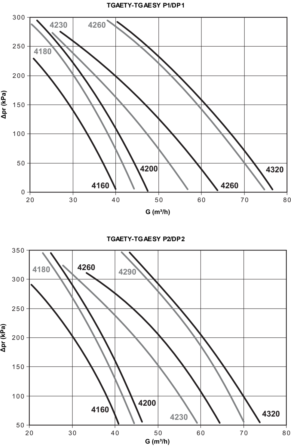
Graph “2”: residual static pressure.
