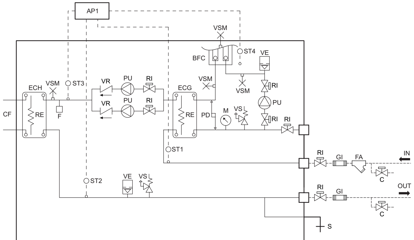
TGAETY - TGAESY Pump DP1/DP2 installation
